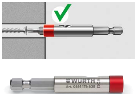
1/4" bit holder, magnetic Art. no. 0614 176 638
