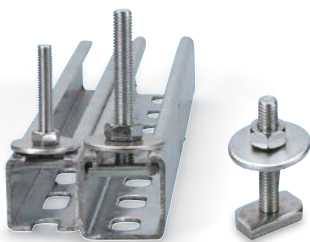
VARIFIX® hammer head fastener, pipe installation Art. no. 08621 000..
