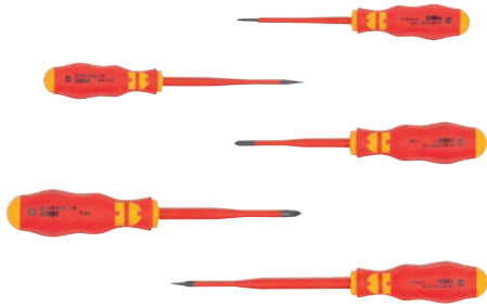
ZEBRA® VDE screwdriver assortment slotted/PH Extra slim design: Five-piece: 1x slotted 0.4 x 2.5; 1x slotted 0.8 x 4.0; 1x slotted 1.0 x 5.5; 1x PH1; 1x PH2 Art. no. 0613 963 250
